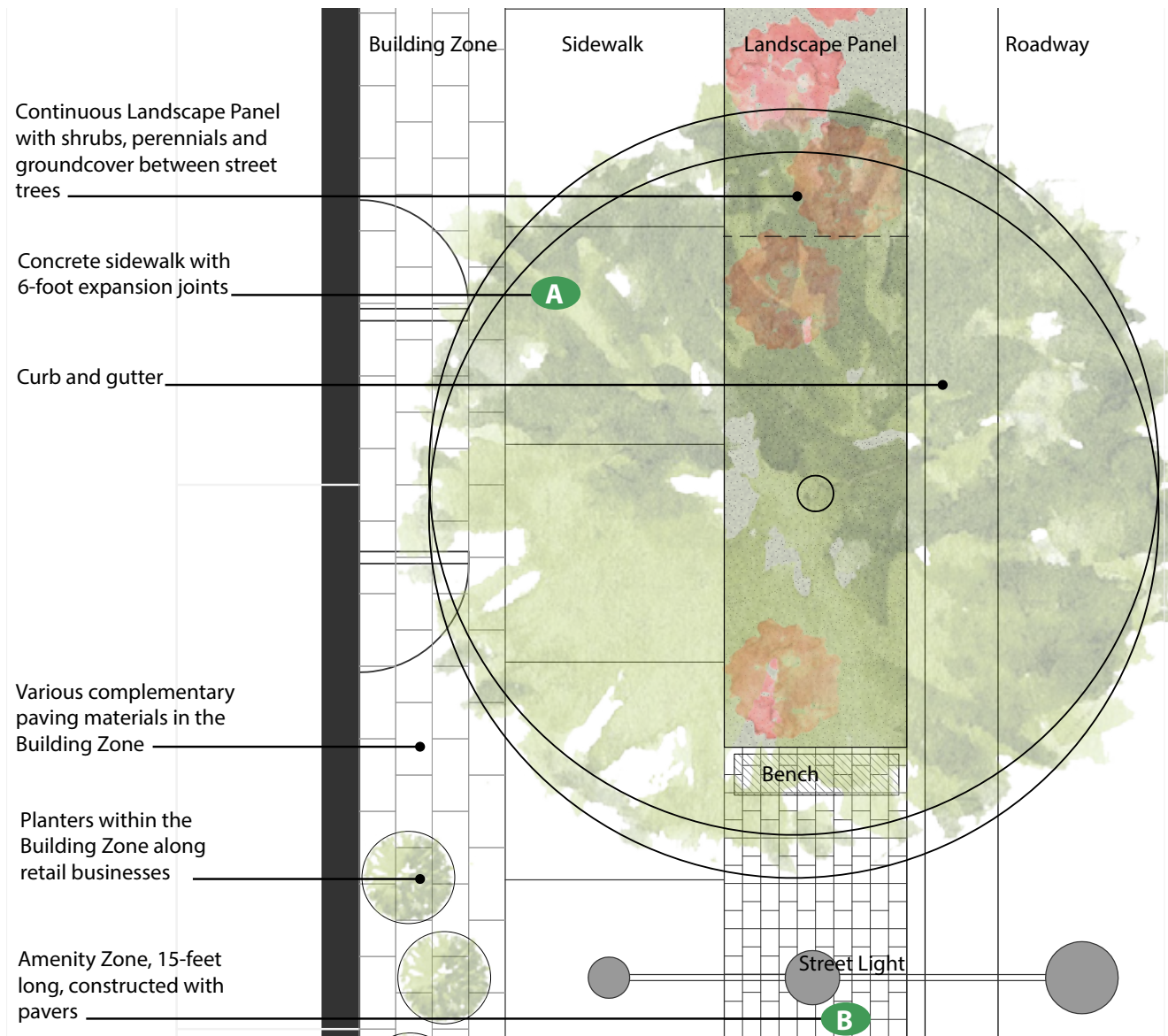
DIAGRAM 2 Depicts the locations of paving materials within streetscape areas; letters correspond to paving specifications listed on page 4-13
